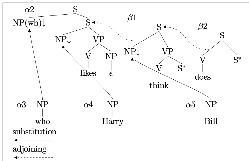
Figure 9: LTAG derivation for who does Bill think Harry likes
