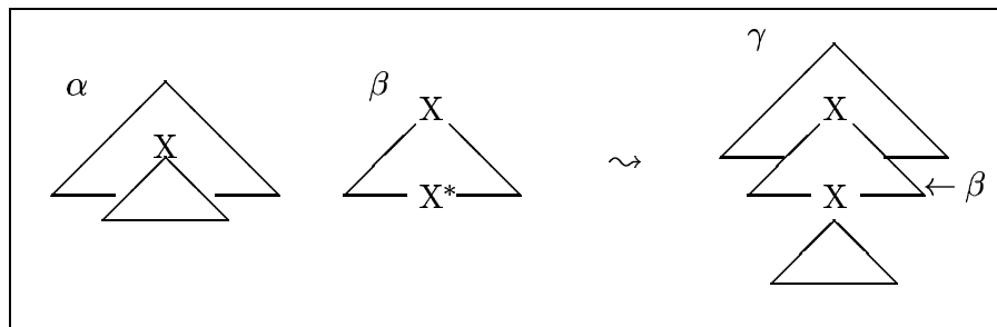
Figure 5: Adjoining
