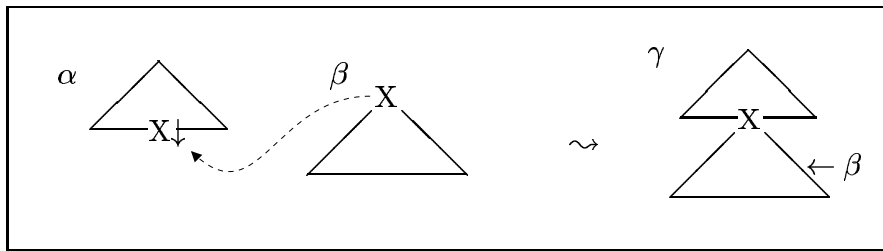
Figure 2: Substitution
