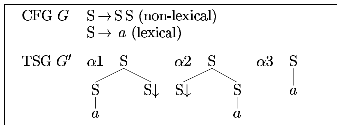
Figure 4: A tree substitution grammar
